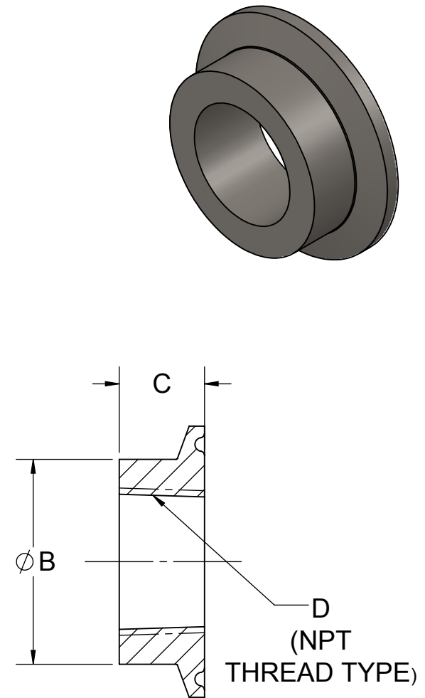
SECTION Z-Z
